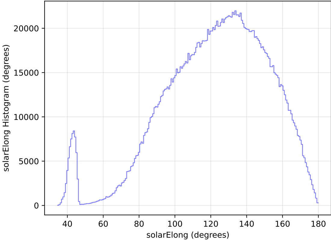
ddf_loaded_fl1_v3.4_10yrs WFD all bands: solarElong Histogram
