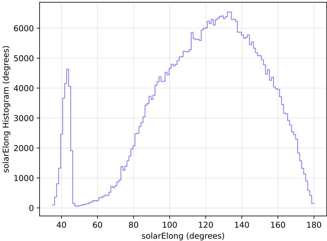
ddf_loaded_fl1_v3.4_10yrs All sky z band: solarElong Histogram
