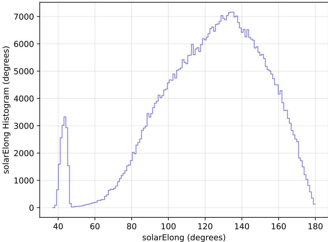
ddf_loaded_fl1_v3.4_10yrs All sky r band: solarElong Histogram
