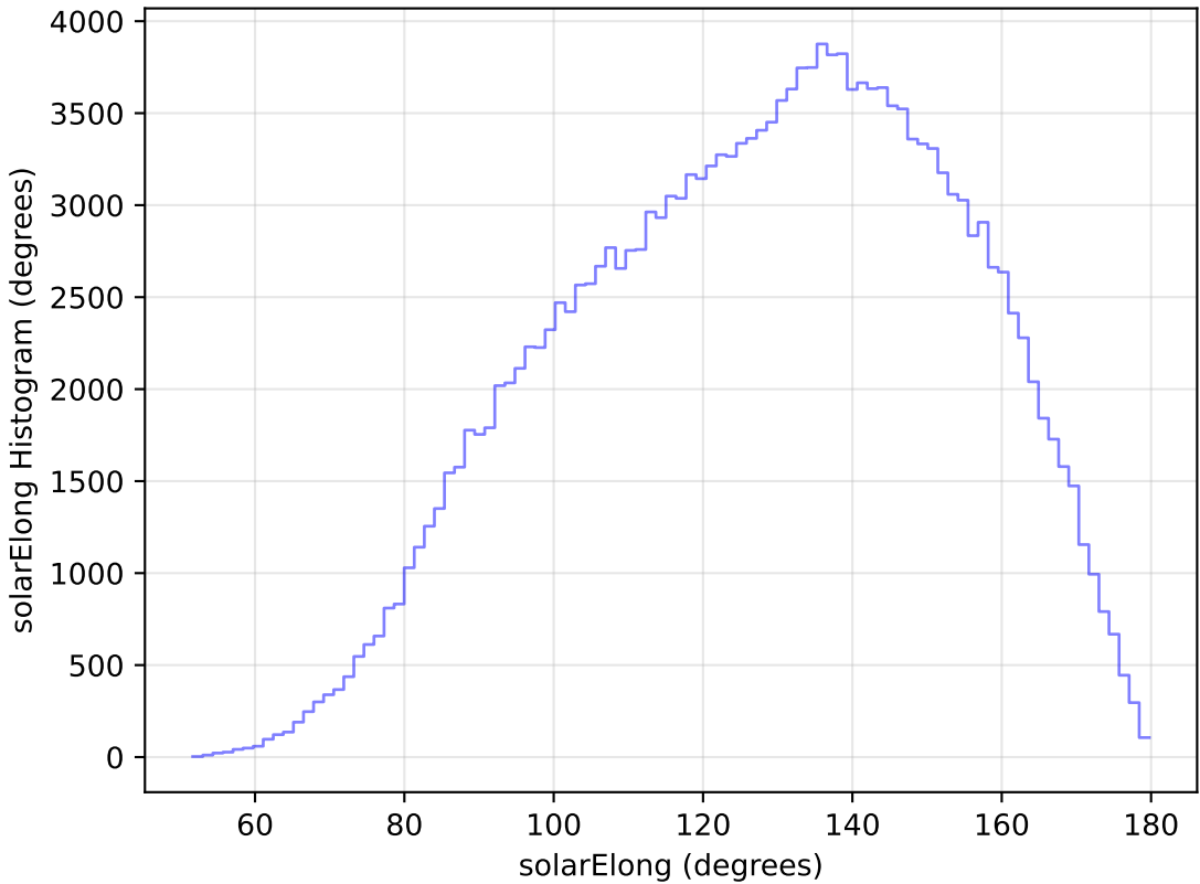
ddf_loaded_fl1_v3.4_10yrs All sky g band: solarElong Histogram
