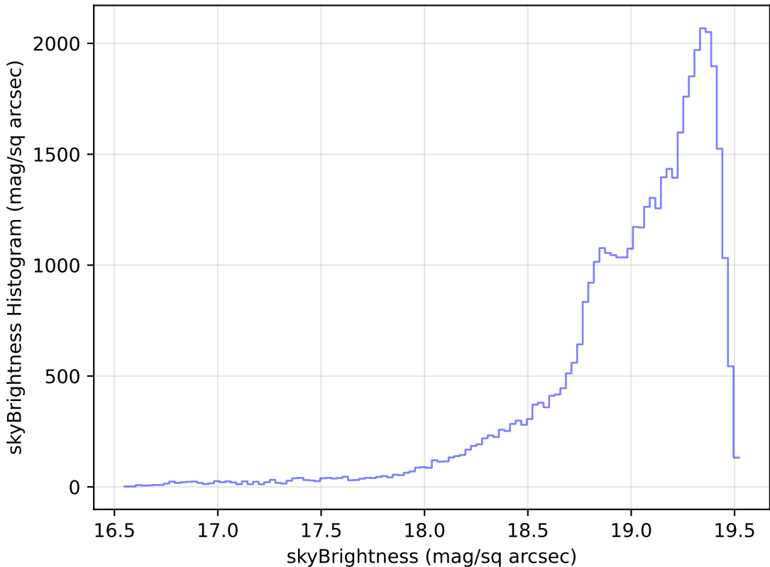
ddf_loaded_fl1_v3.4_10yrs Yr 1 z band: skyBrightness Histogram
