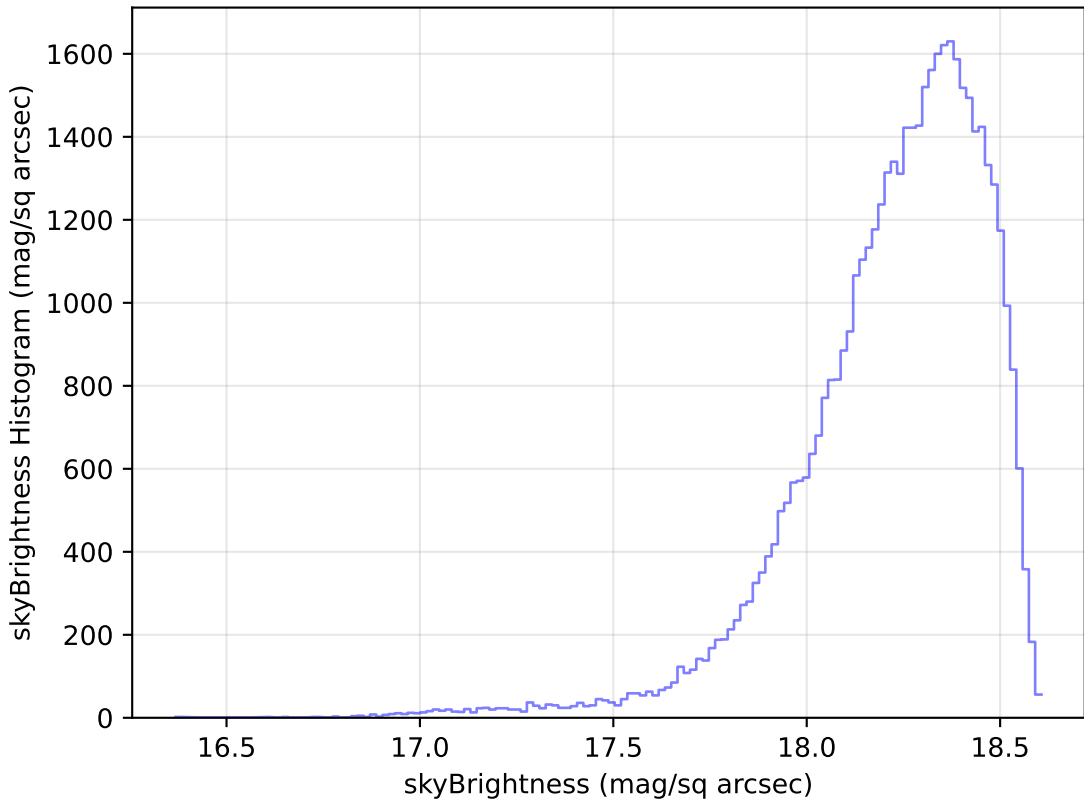
ddf_loaded_fl1_v3.4_10yrs Yr 1 y band: skyBrightness Histogram
