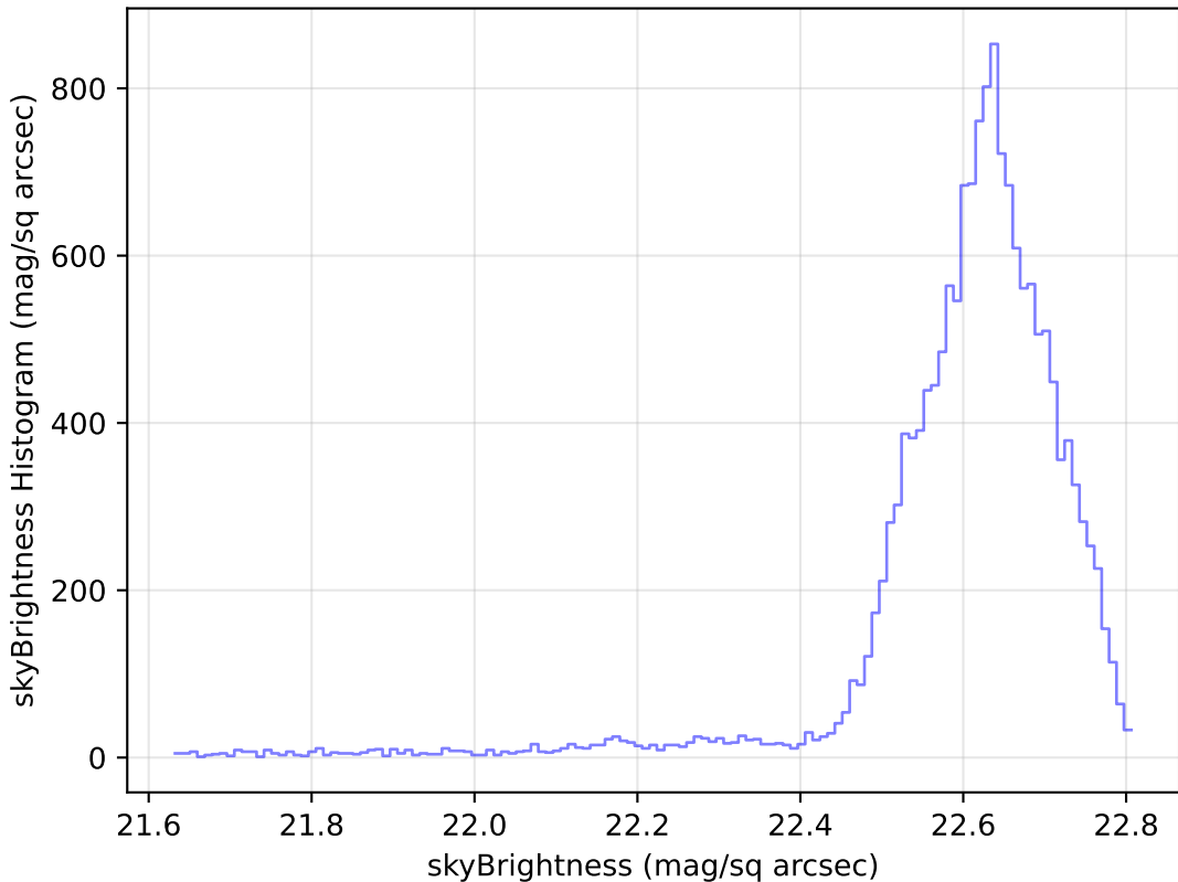
ddf_loaded_fl1_v3.4_10yrs Yr 1 u band: skyBrightness Histogram
