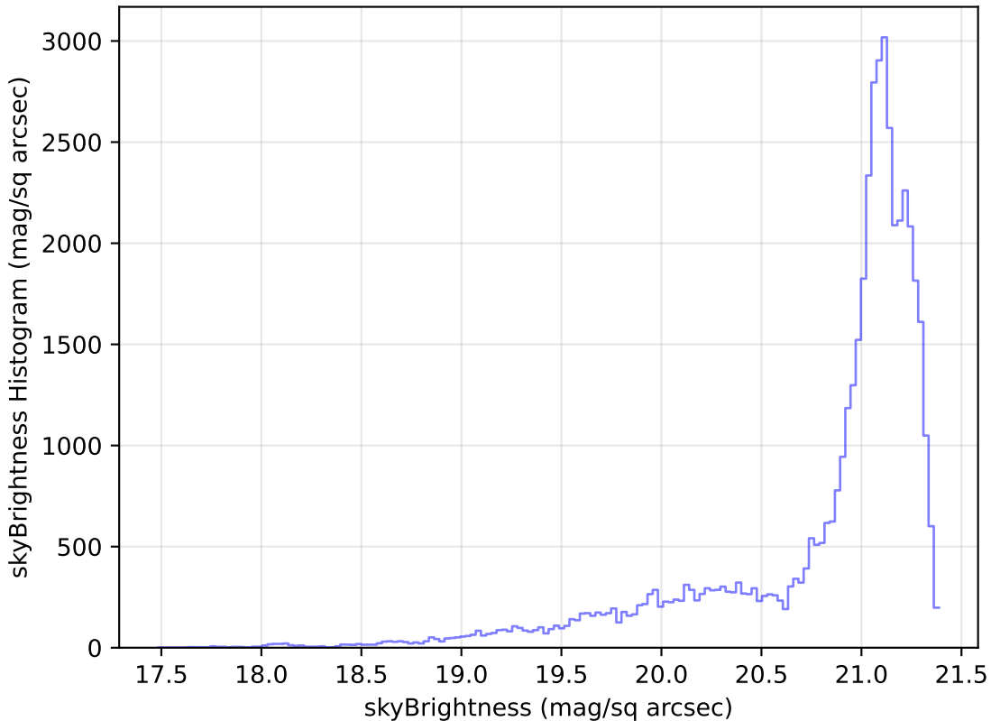
ddf_loaded_fl1_v3.4_10yrs Yr 1 r band: skyBrightness Histogram
