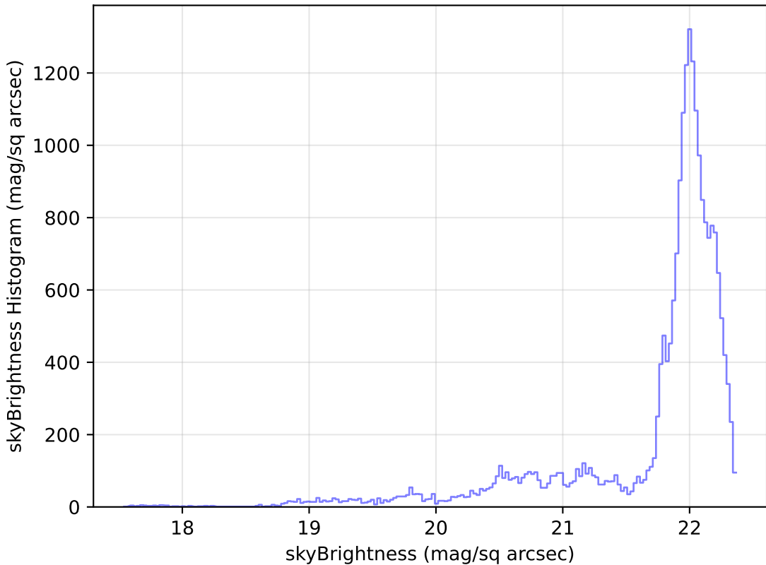
ddf_loaded_fl1_v3.4_10yrs Yr 1 g band: skyBrightness Histogram
