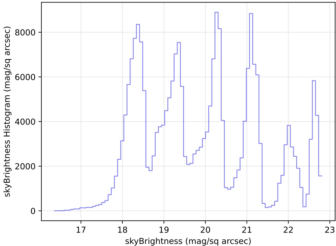
ddf_loaded_fl1_v3.4_10yrs Yr 1 all bands: skyBrightness Histogram
