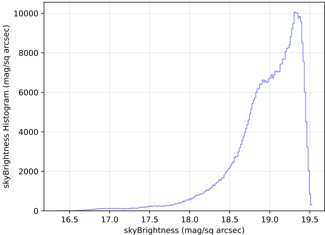
ddf_loaded_fl1_v3.4_10yrs WFD z band: skyBrightness Histogram
