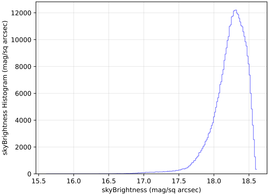
ddf_loaded_fl1_v3.4_10yrs WFD y band: skyBrightness Histogram
