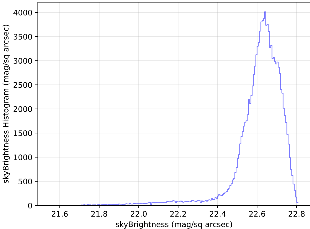
ddf_loaded_fl1_v3.4_10yrs WFD u band: skyBrightness Histogram
