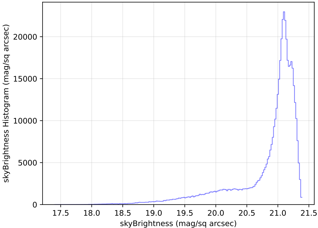
ddf_loaded_fl1_v3.4_10yrs WFD r band: skyBrightness Histogram
