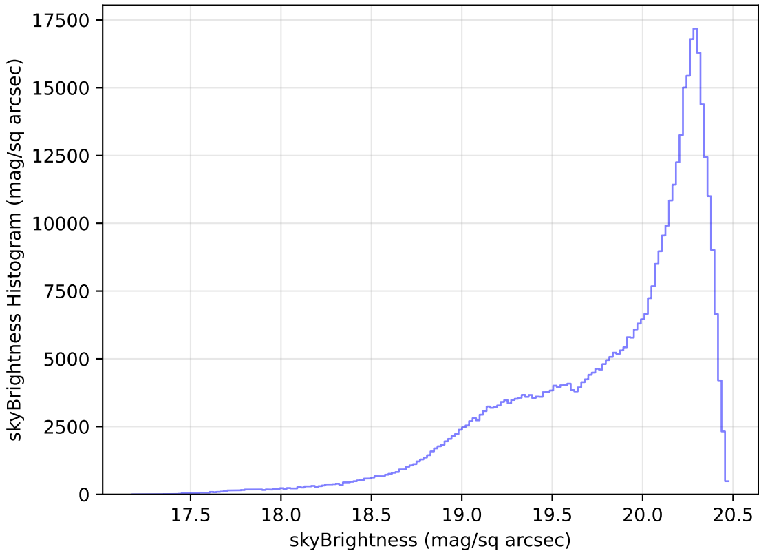
ddf_loaded_fl1_v3.4_10yrs WFD i band: skyBrightness Histogram
