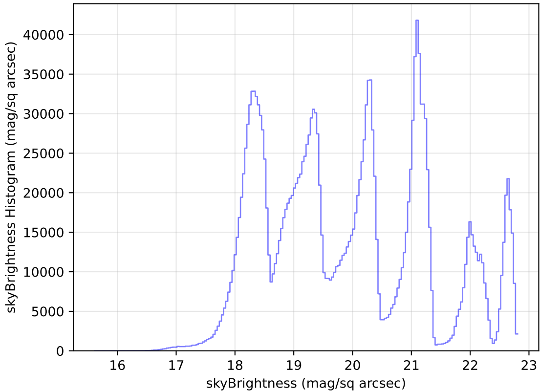
ddf_loaded_fl1_v3.4_10yrs WFD all bands: skyBrightness Histogram
