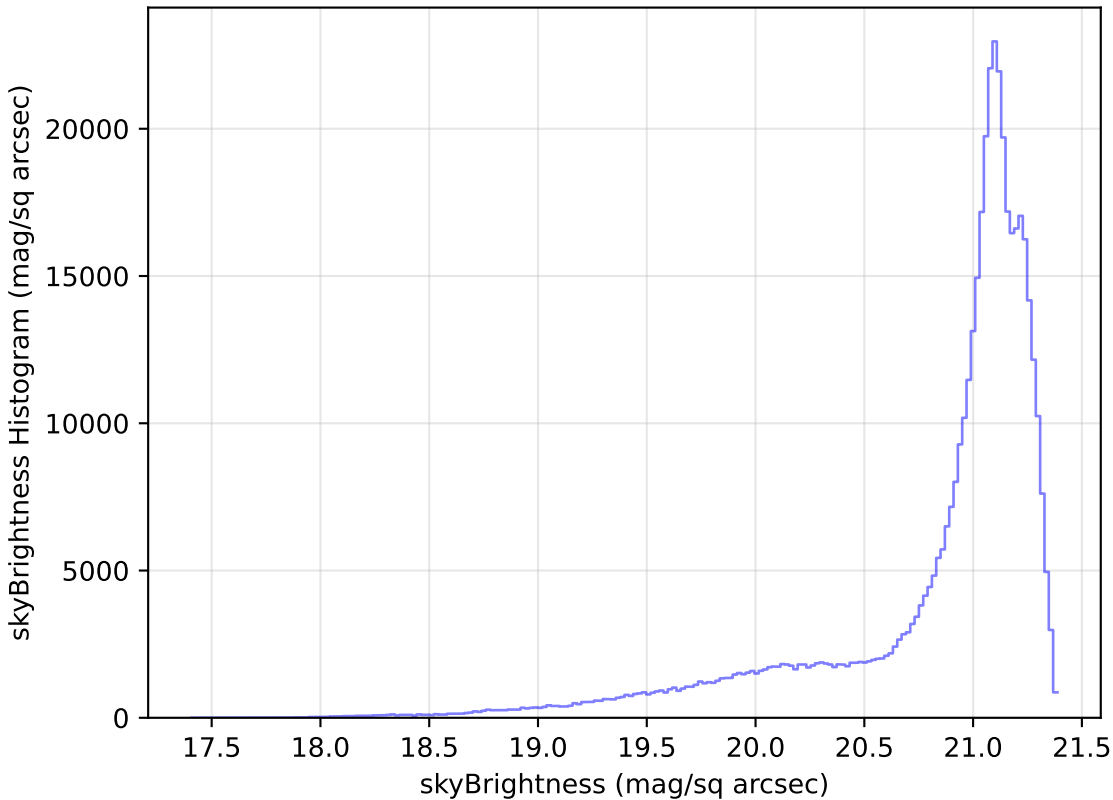
ddf_loaded_fl1_v3.4_10yrs All sky r band: skyBrightness Histogram
