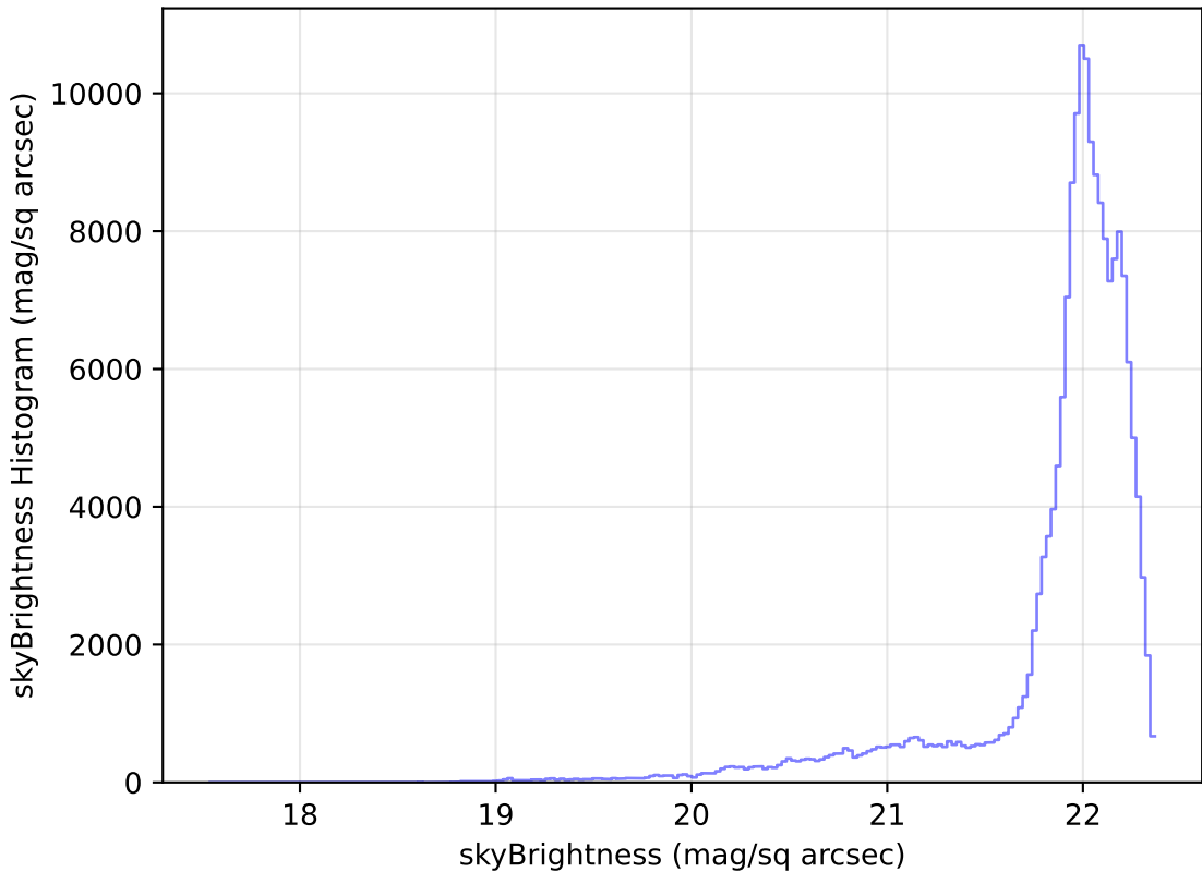
ddf_loaded_fl1_v3.4_10yrs All sky g band: skyBrightness Histogram
