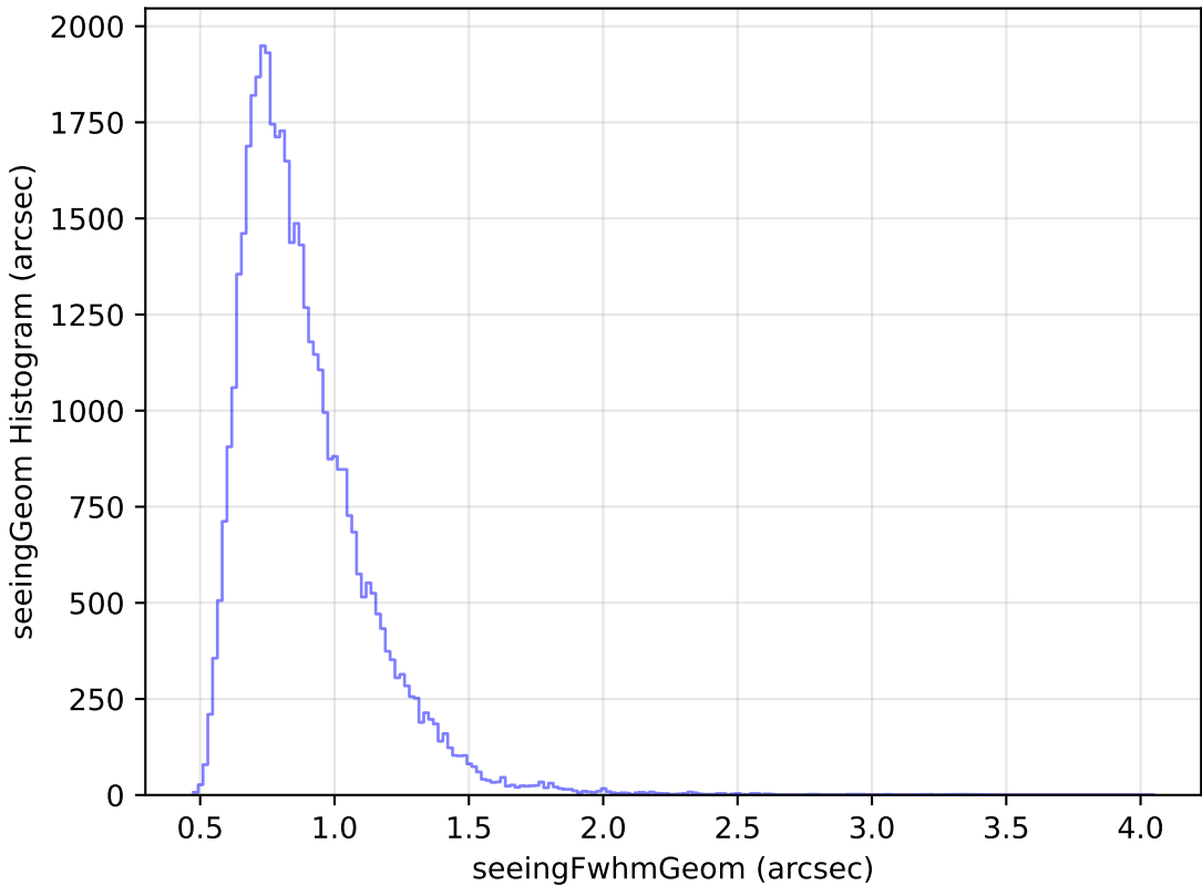
ddf_loaded_fl1_v3.4_10yrs Yr 1 z band: seeingGeom Histogram
