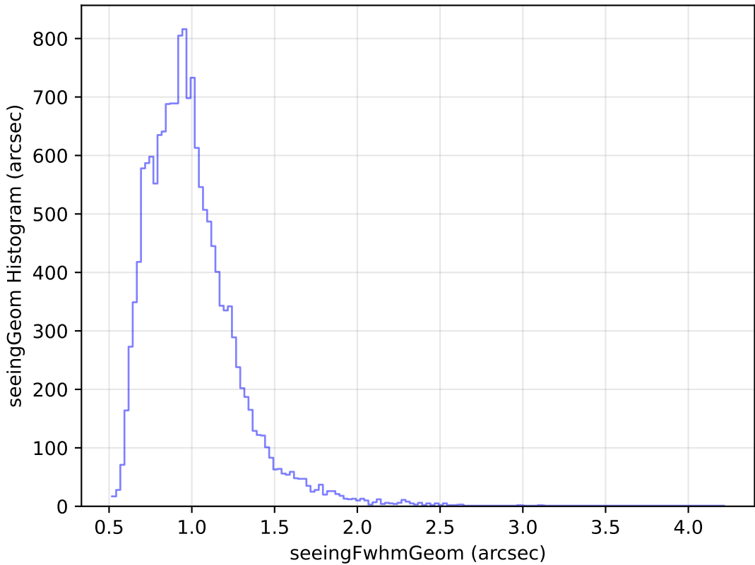
ddf_loaded_fl1_v3.4_10yrs Yr 1 u band: seeingGeom Histogram
