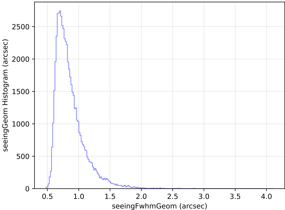
ddf_loaded_fl1_v3.4_10yrs Yr 1 i band: seeingGeom Histogram
