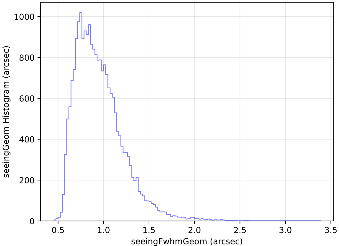
ddf_loaded_fl1_v3.4_10yrs Yr 1 g band: seeingGeom Histogram
