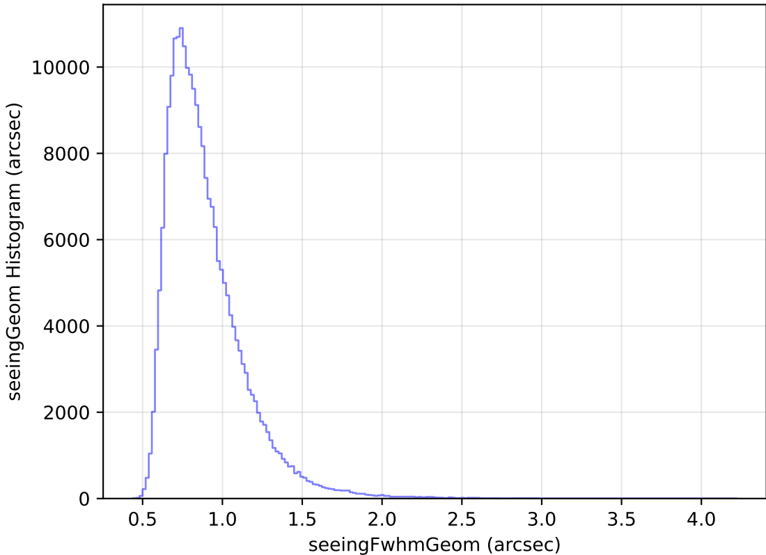
ddf_loaded_fl1_v3.4_10yrs Yr 1 all bands: seeingGeom Histogram
