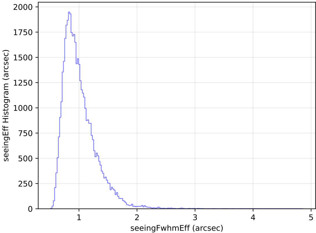
ddf_loaded_fl1_v3.4_10yrs Yr 1 z band: seeingEff Histogram
