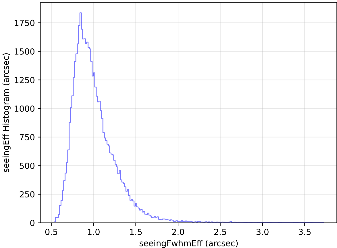
ddf_loaded_fl1_v3.4_10yrs Yr 1 y band: seeingEff Histogram
