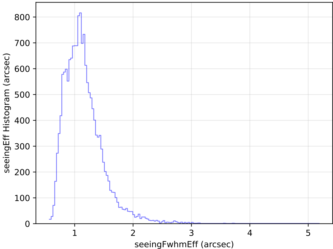
ddf_loaded_fl1_v3.4_10yrs Yr 1 u band: seeingEff Histogram
