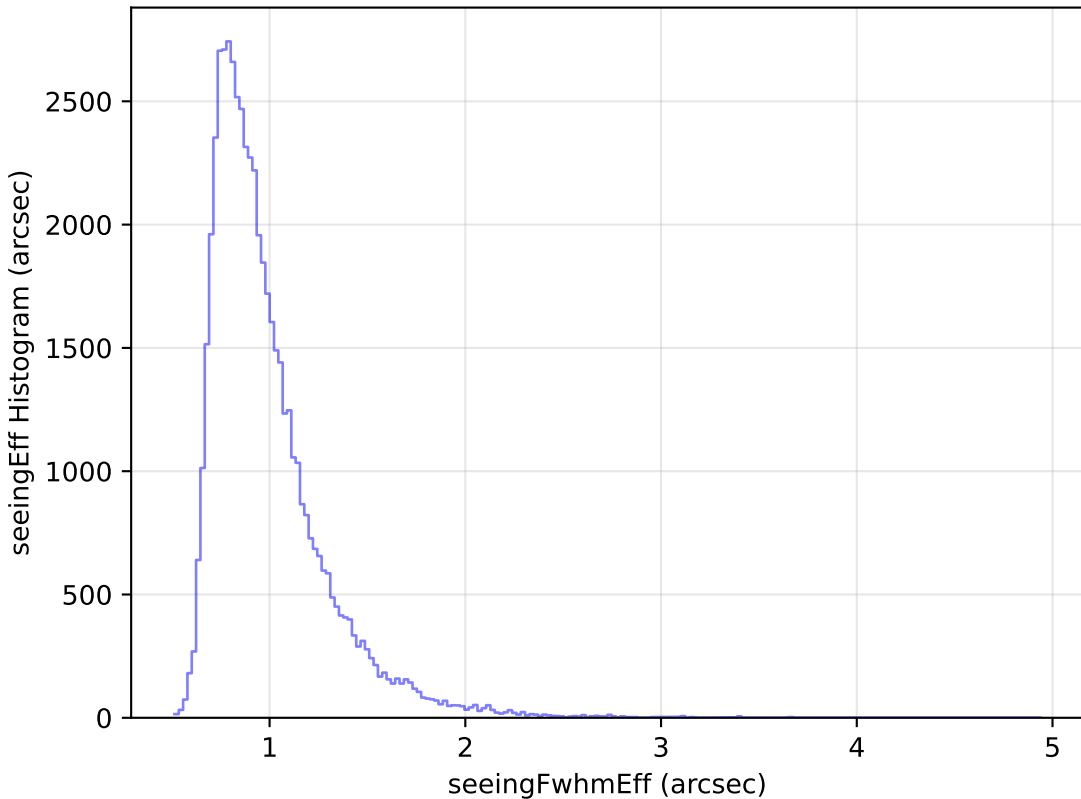
ddf_loaded_fl1_v3.4_10yrs Yr 1 i band: seeingEff Histogram
