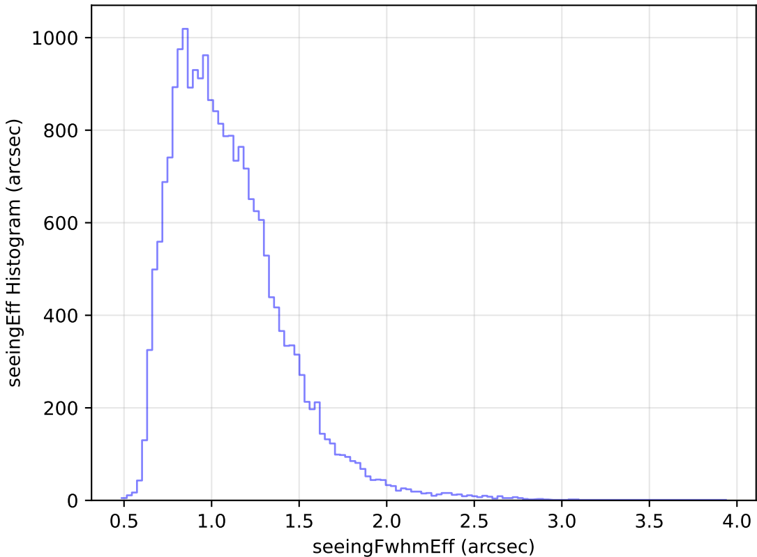
ddf_loaded_fl1_v3.4_10yrs Yr 1 g band: seeingEff Histogram
