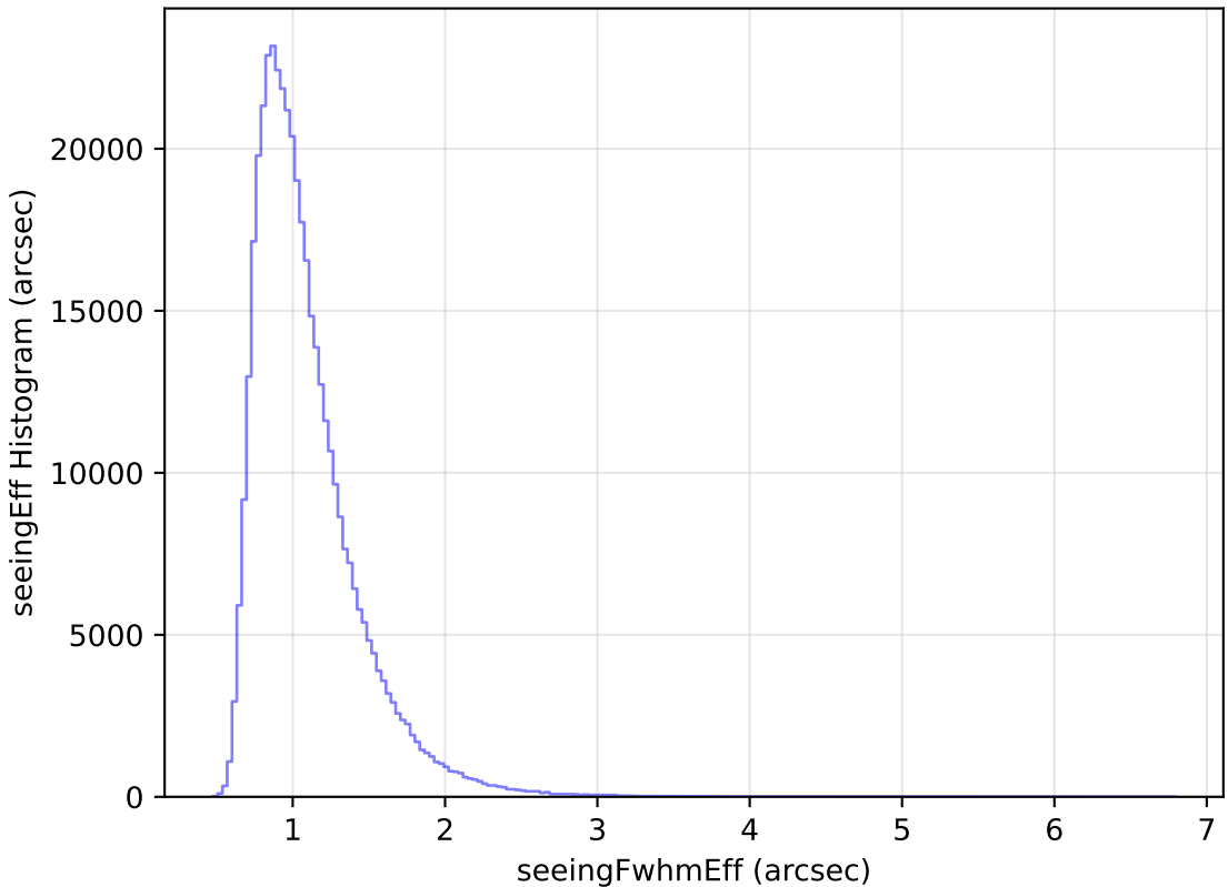
ddf_loaded_fl1_v3.4_10yrs WFD z band: seeingEff Histogram
