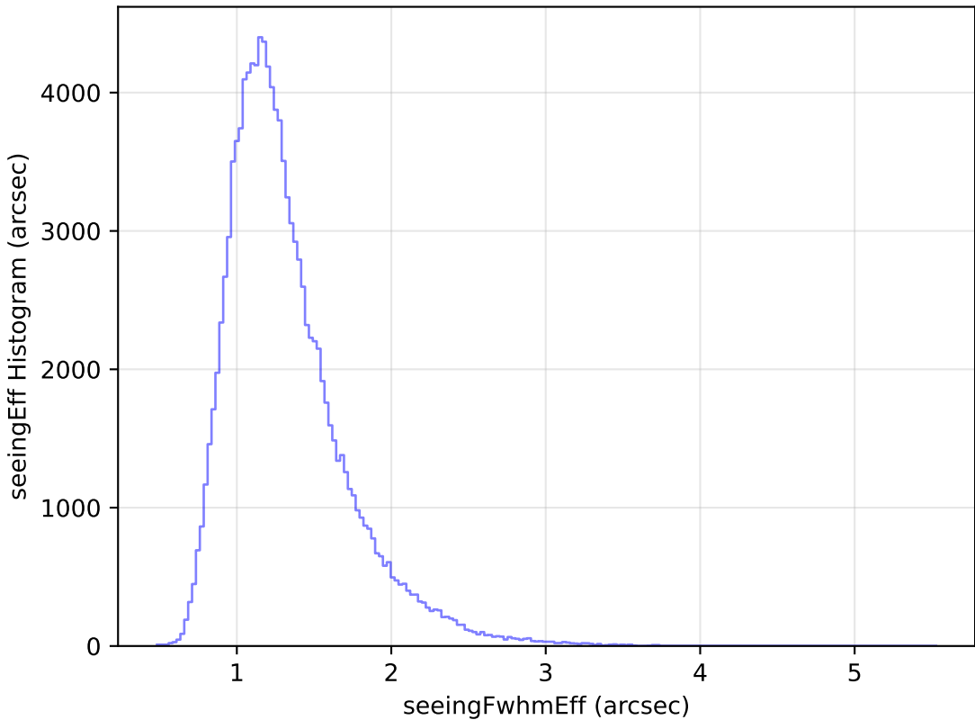
ddf_loaded_fl1_v3.4_10yrs WFD u band: seeingEff Histogram
