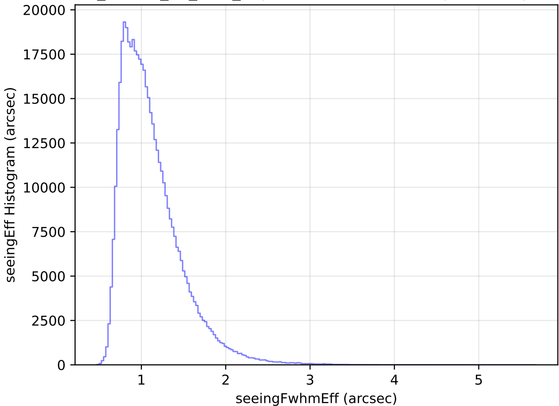
ddf_loaded_fl1_v3.4_10yrs WFD r band: seeingEff Histogram
