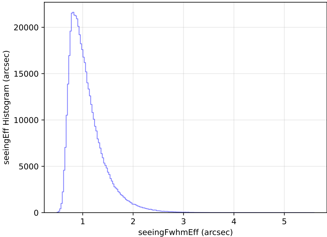
ddf_loaded_fl1_v3.4_10yrs WFD i band: seeingEff Histogram
