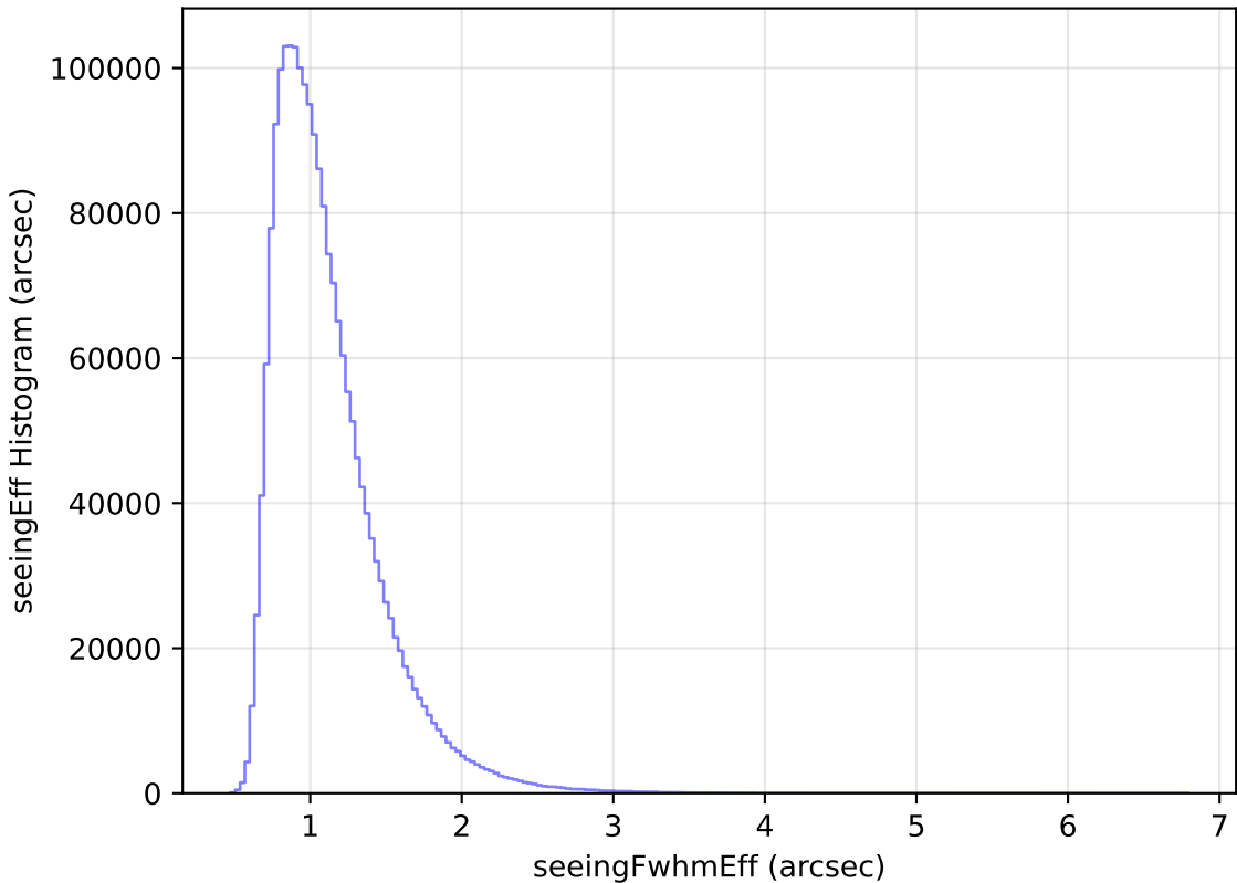
ddf_loaded_fl1_v3.4_10yrs WFD all bands: seeingEff Histogram
