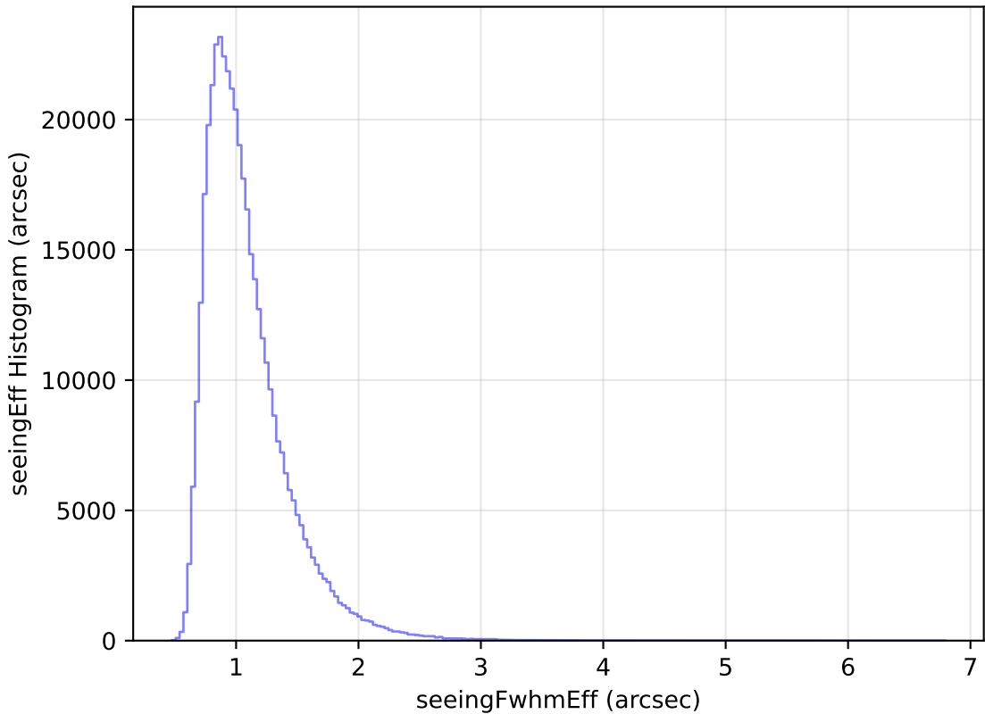
ddf_loaded_fl1_v3.4_10yrs All sky z band: seeingEff Histogram
