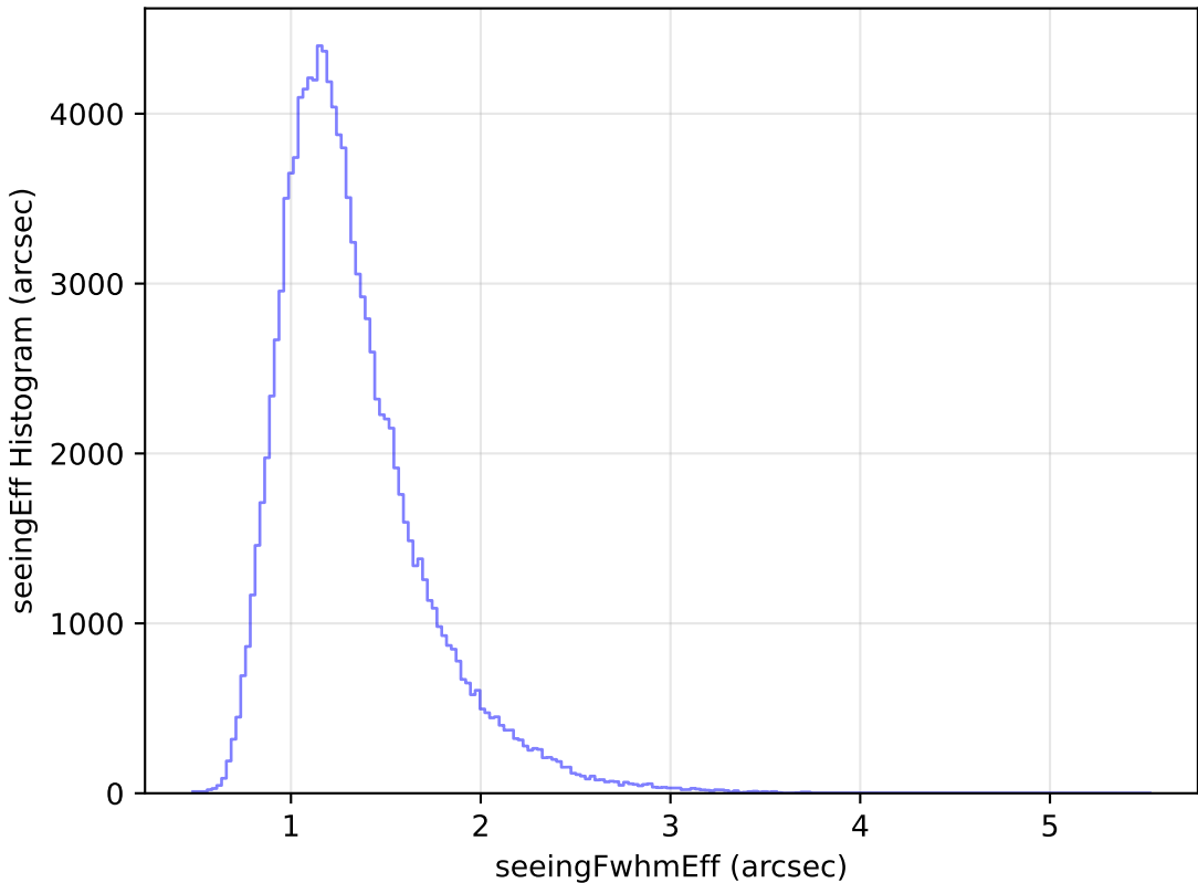
ddf_loaded_fl1_v3.4_10yrs All sky u band: seeingEff Histogram
