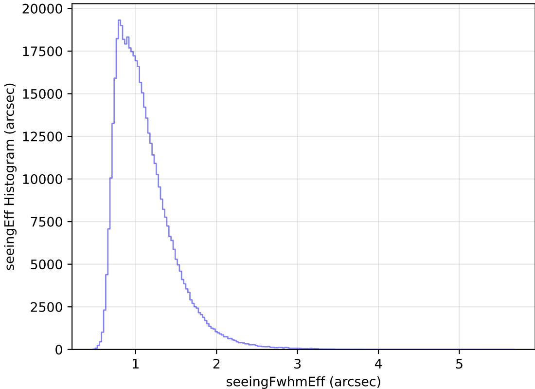
ddf_loaded_fl1_v3.4_10yrs All sky r band: seeingEff Histogram
