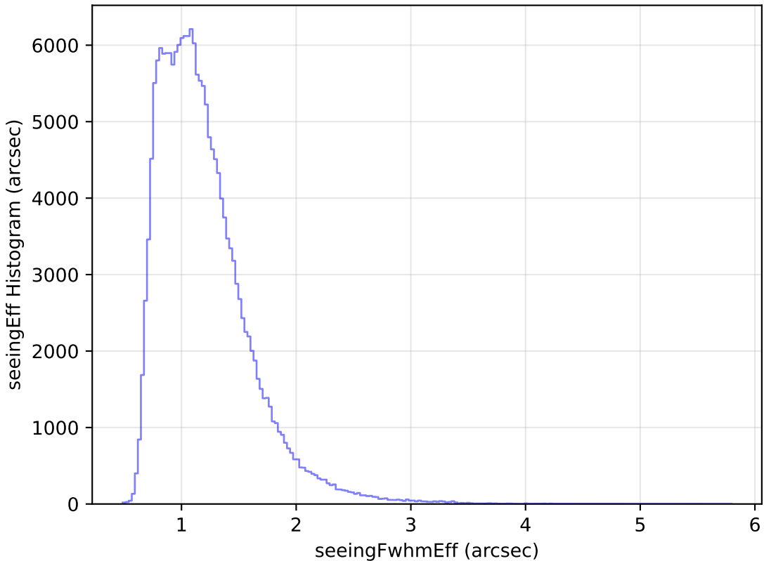
ddf_loaded_fl1_v3.4_10yrs All sky g band: seeingEff Histogram
