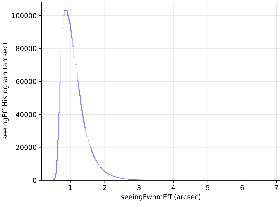
ddf_loaded_fl1_v3.4_10yrs All sky all bands: seeingEff Histogram
