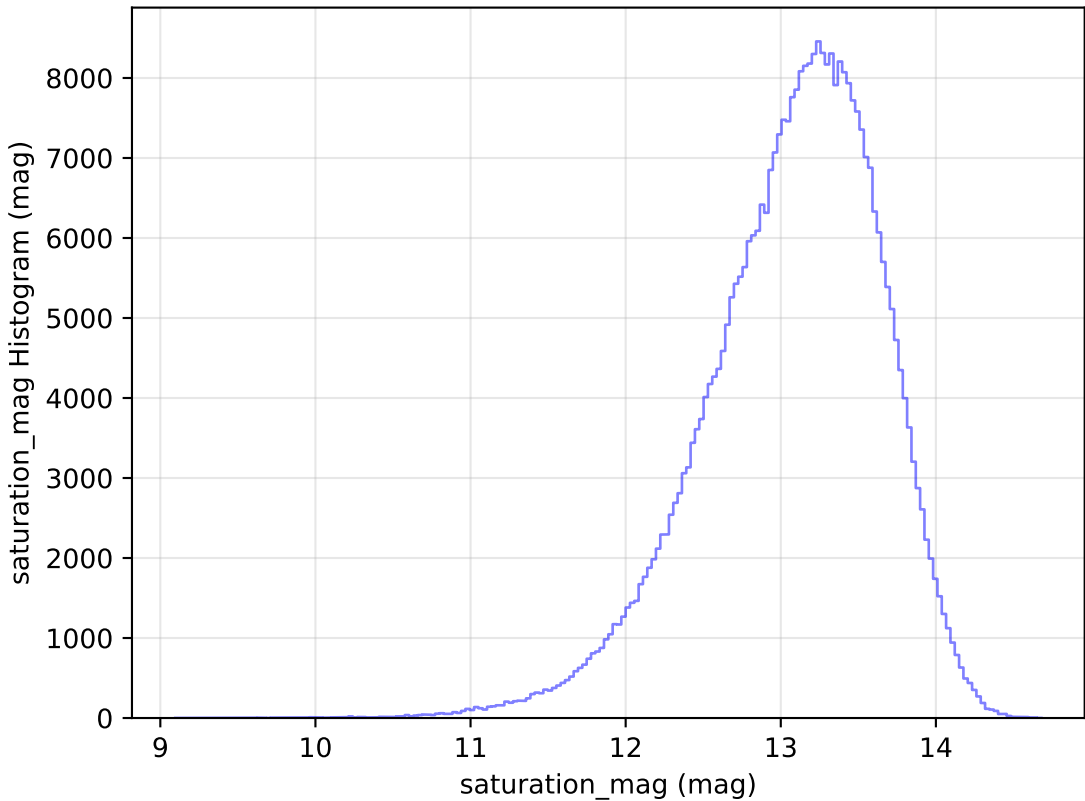
ddf_loaded_fl1_v3.4_10yrs WFD y band: saturation_mag Histogram
