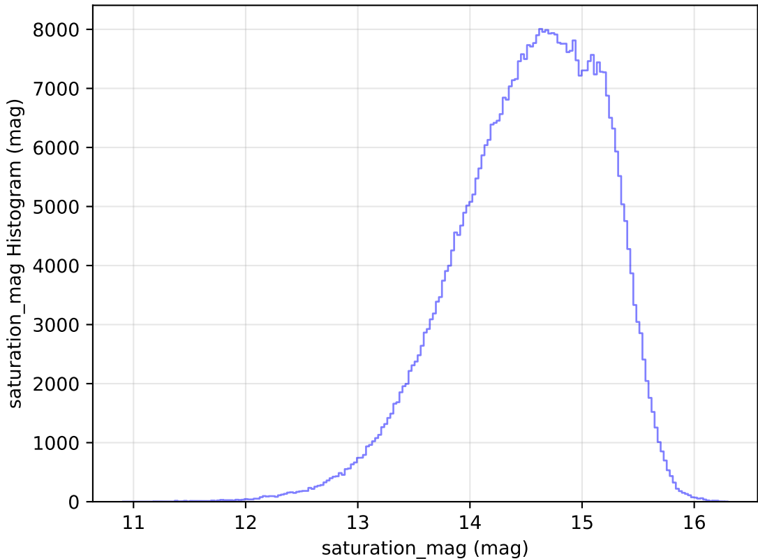
ddf_loaded_fl1_v3.4_10yrs WFD r band: saturation_mag Histogram
