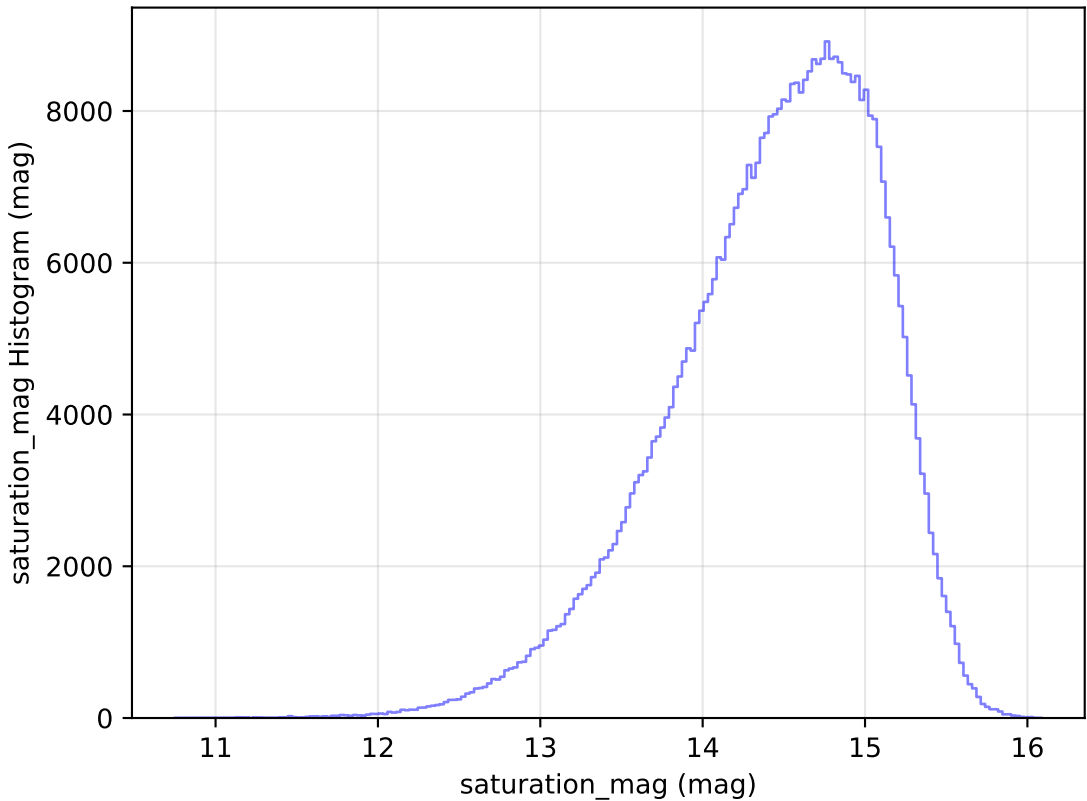
ddf_loaded_fl1_v3.4_10yrs WFD i band: saturation_mag Histogram
