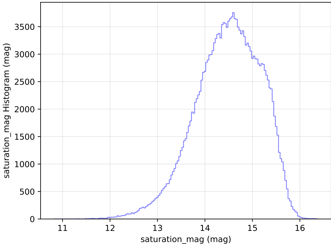
ddf_loaded_fl1_v3.4_10yrs WFD g band: saturation_mag Histogram
