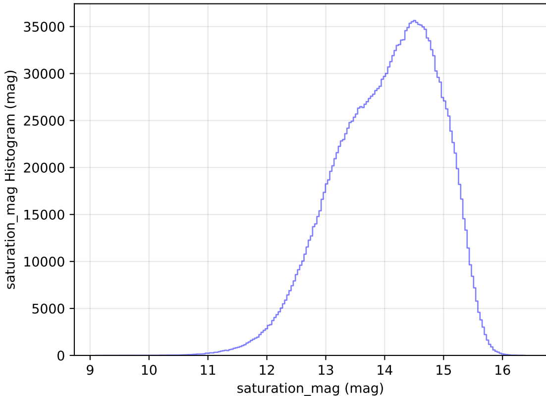
ddf_loaded_fl1_v3.4_10yrs WFD all bands: saturation_mag Histogram
