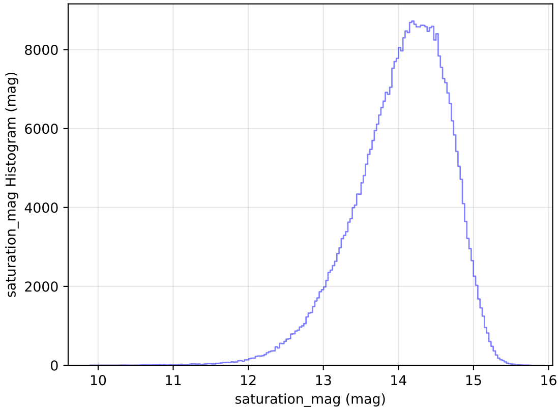
ddf_loaded_fl1_v3.4_10yrs All sky z band: saturation_mag Histogram
