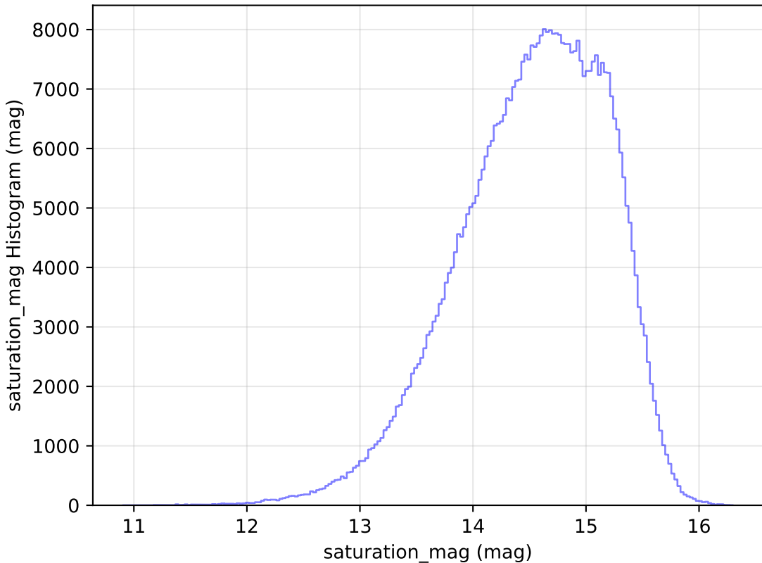
ddf_loaded_fl1_v3.4_10yrs All sky r band: saturation_mag Histogram
