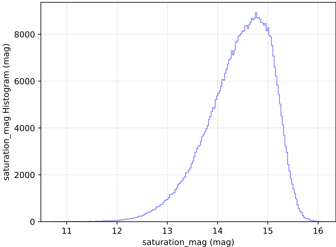
ddf_loaded_fl1_v3.4_10yrs All sky i band: saturation_mag Histogram
