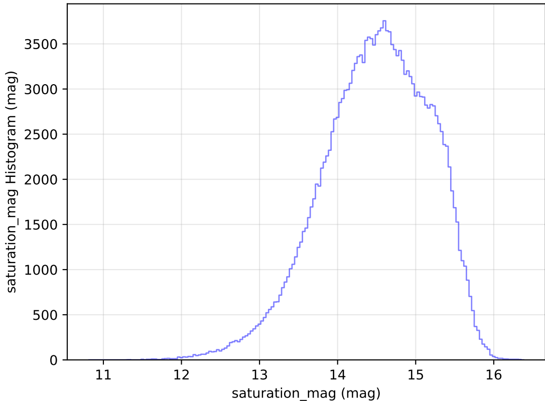
ddf_loaded_fl1_v3.4_10yrs All sky g band: saturation_mag Histogram
