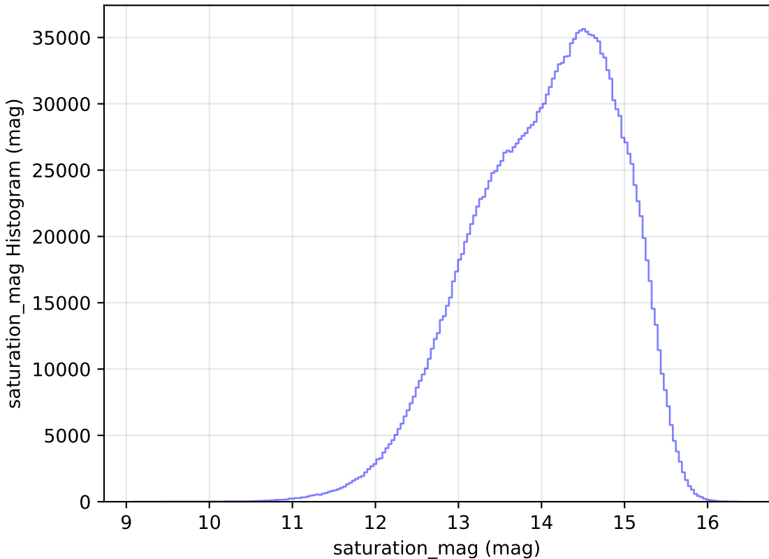
ddf_loaded_fl1_v3.4_10yrs All sky all bands: saturation_mag Histogram
