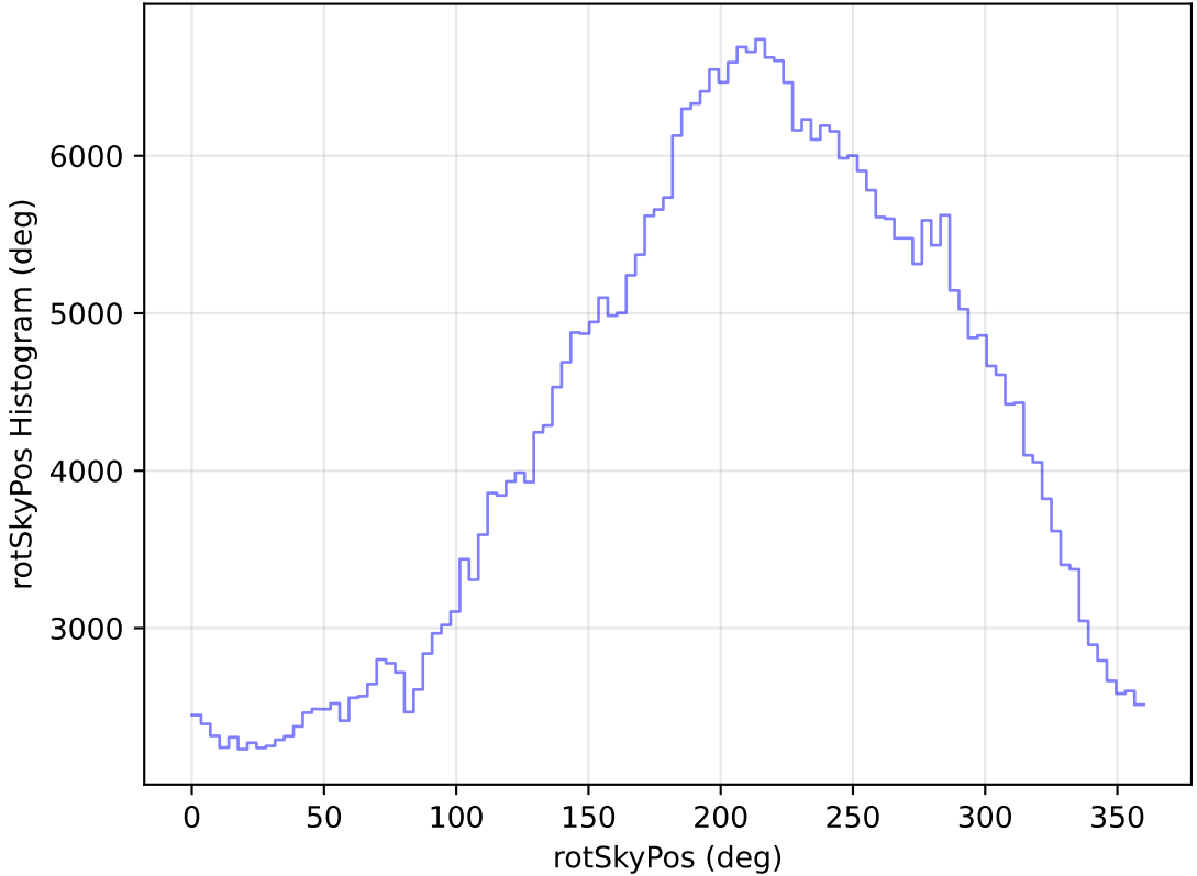
ddf_loaded_fl1_v3.4_10yrs WFD z band: rotSkyPos Histogram
