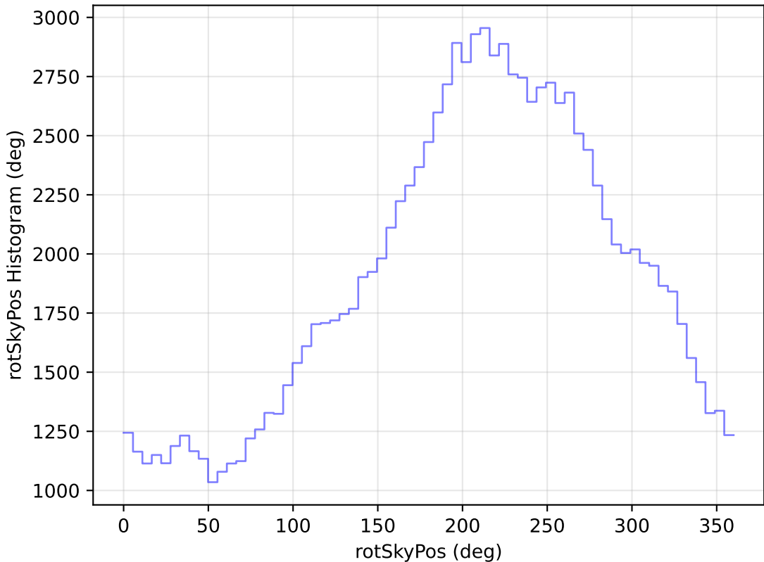
ddf_loaded_fl1_v3.4_10yrs WFD u band: rotSkyPos Histogram
